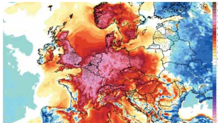
Tue, July 19, 2022 (noon GMT) temperatures were transcending average values for the time of day and season by 12 to 24 degrees Celsius
